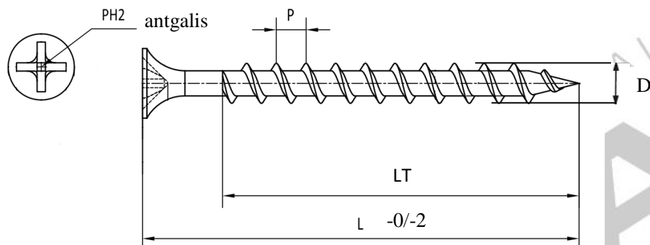
Matmenys/Dimensions mm
