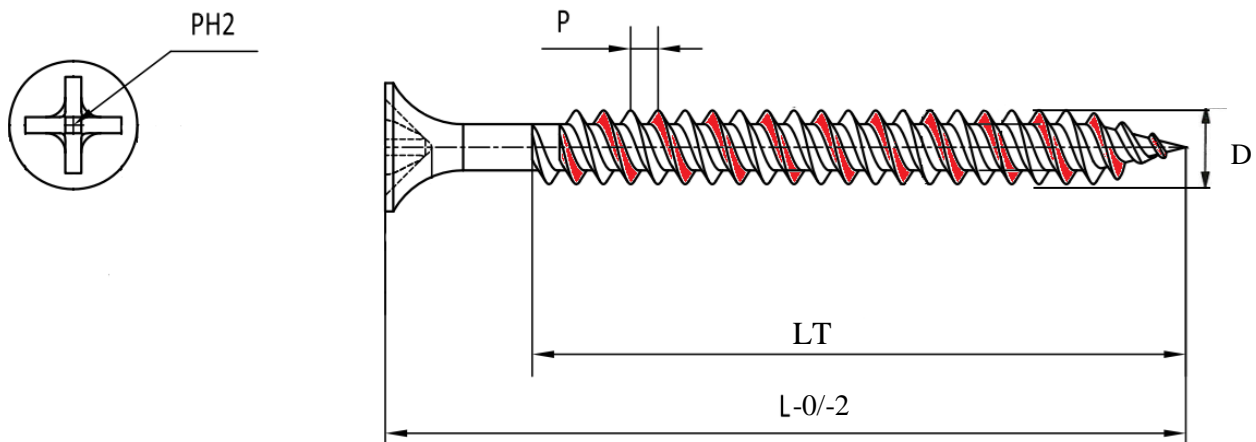
Matmenys/Dimensions mm
