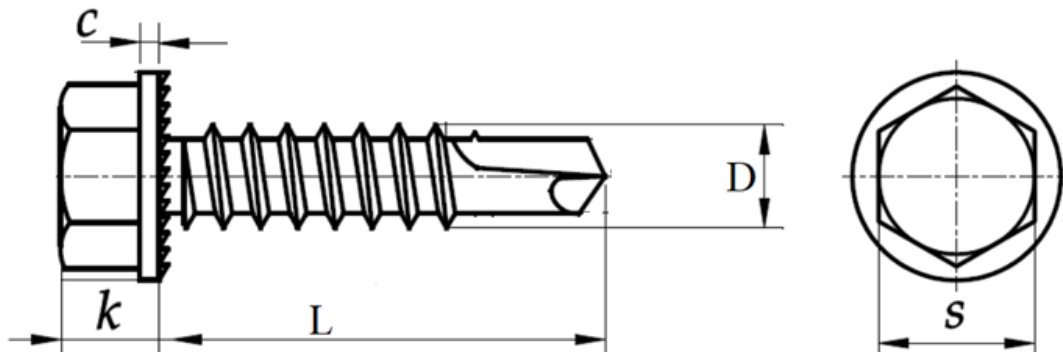
Matmenys/Dimensions
