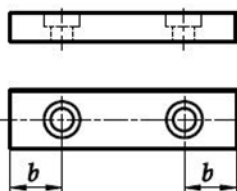
Forma F Stačiakampis su dviem skylėm square ended with holes for 2 retaining screws 8x7 ir 10x8 8x7 and 10x8 nuo 12x8 su papildoma skylė from 12x8 additionally with jacking hole
