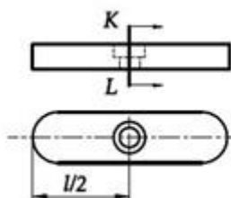
Forma E Apvaliais galais ir dviem skylėm 2 round ended with holes for 2 retaining screws 8x7 ir 10x8 8x7 and 10x8 nuo 12x8 su papildoma skylė from 12x8 additionally with jacking hole
