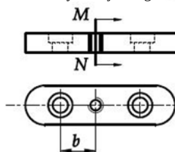
Forma F Stačiakampis su dviem skylėm square ended with holes for 2 retaining screws 8x7 ir 10x8 8x7 and 10x8 nuo 12x8 su papildoma skylė from 12x8 additionally with jacking hole
