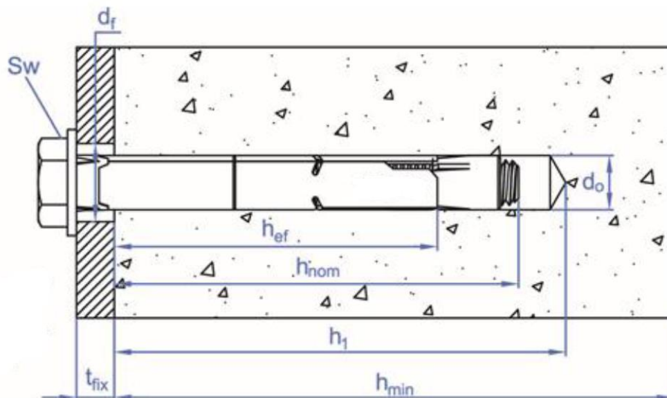
Matmenys/Dimensions
