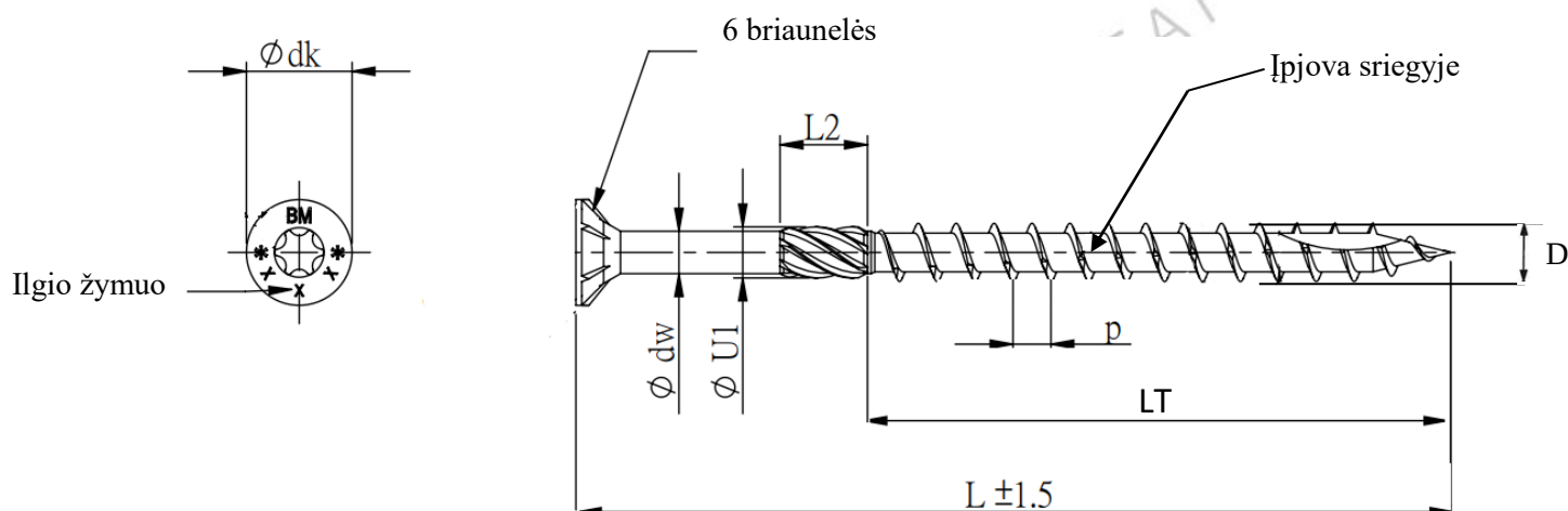
Matmenys/Dimensions, mm
