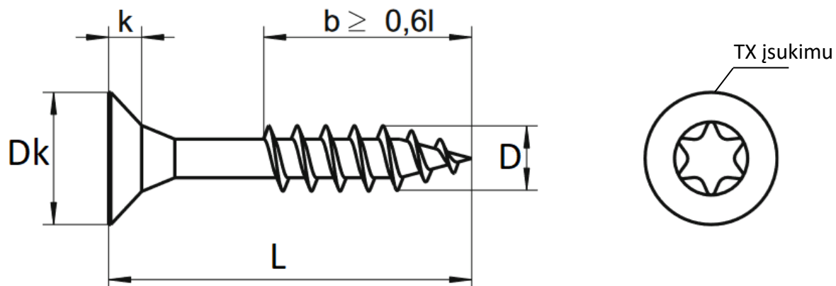
Matmenys/Dimensions
