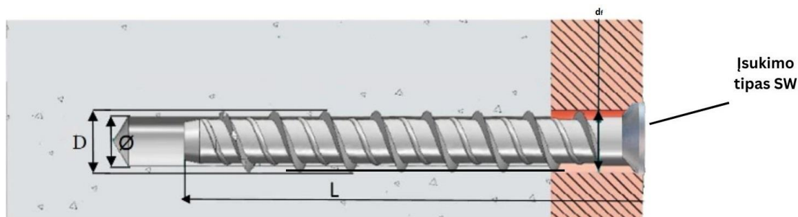
Matmenys/Dimensions mm
