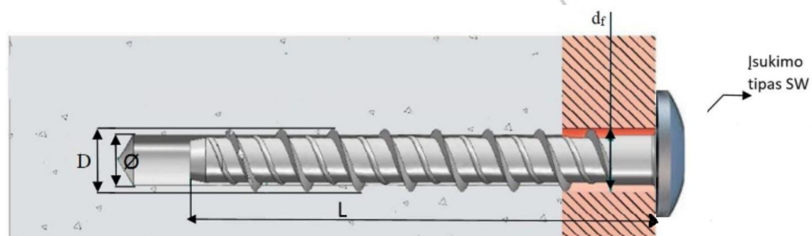
Matmenys/Dimensions mm
