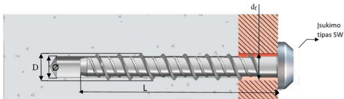
Matmenys/Dimensions mm
