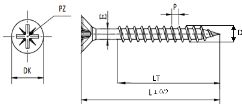
Matmenys/Dimensions mm
