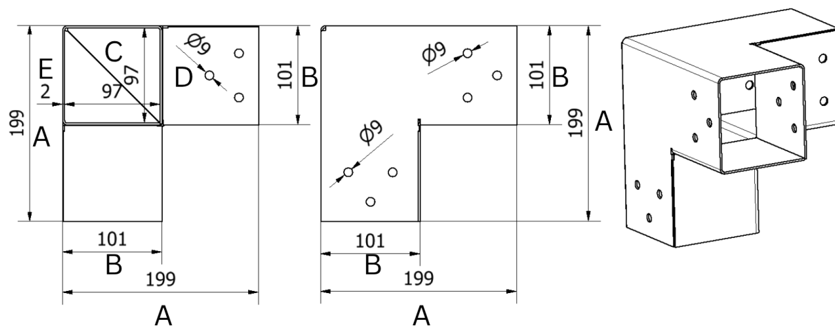
Matmenys/Dimensions, mm
