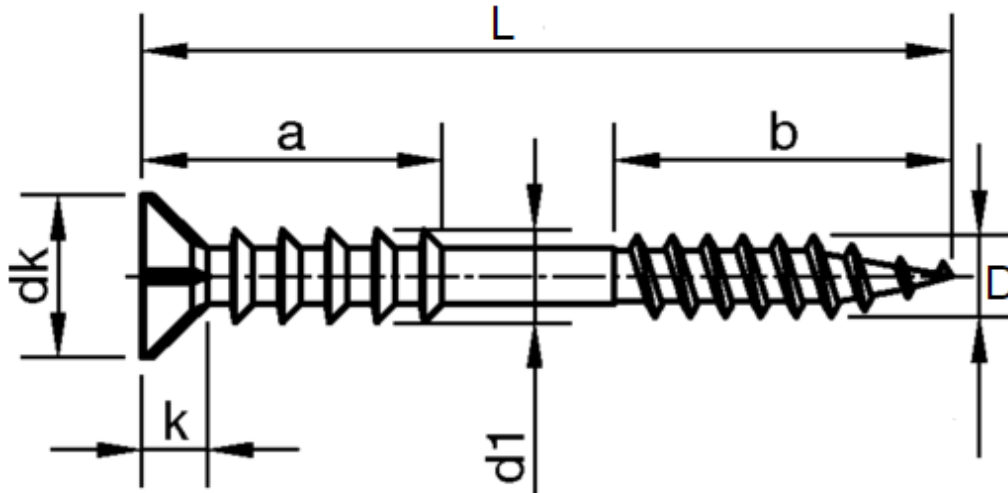
Matmenys/Dimensions mm
